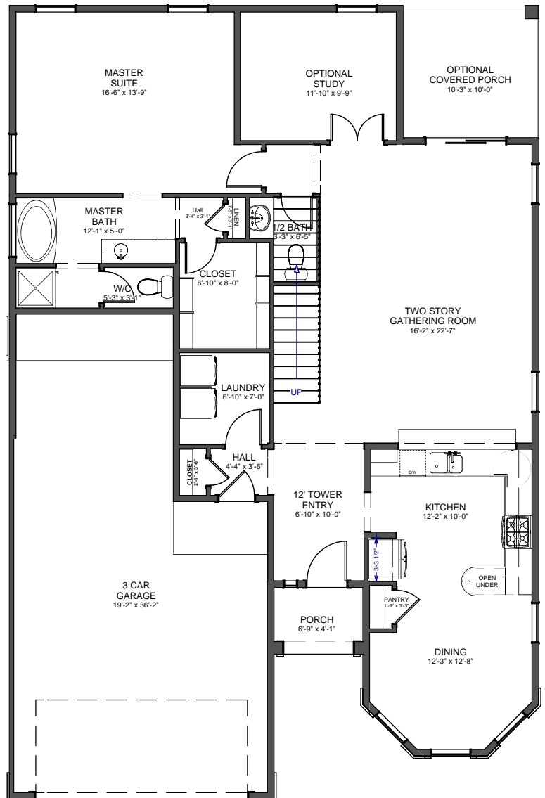
FIRST FLOOR
